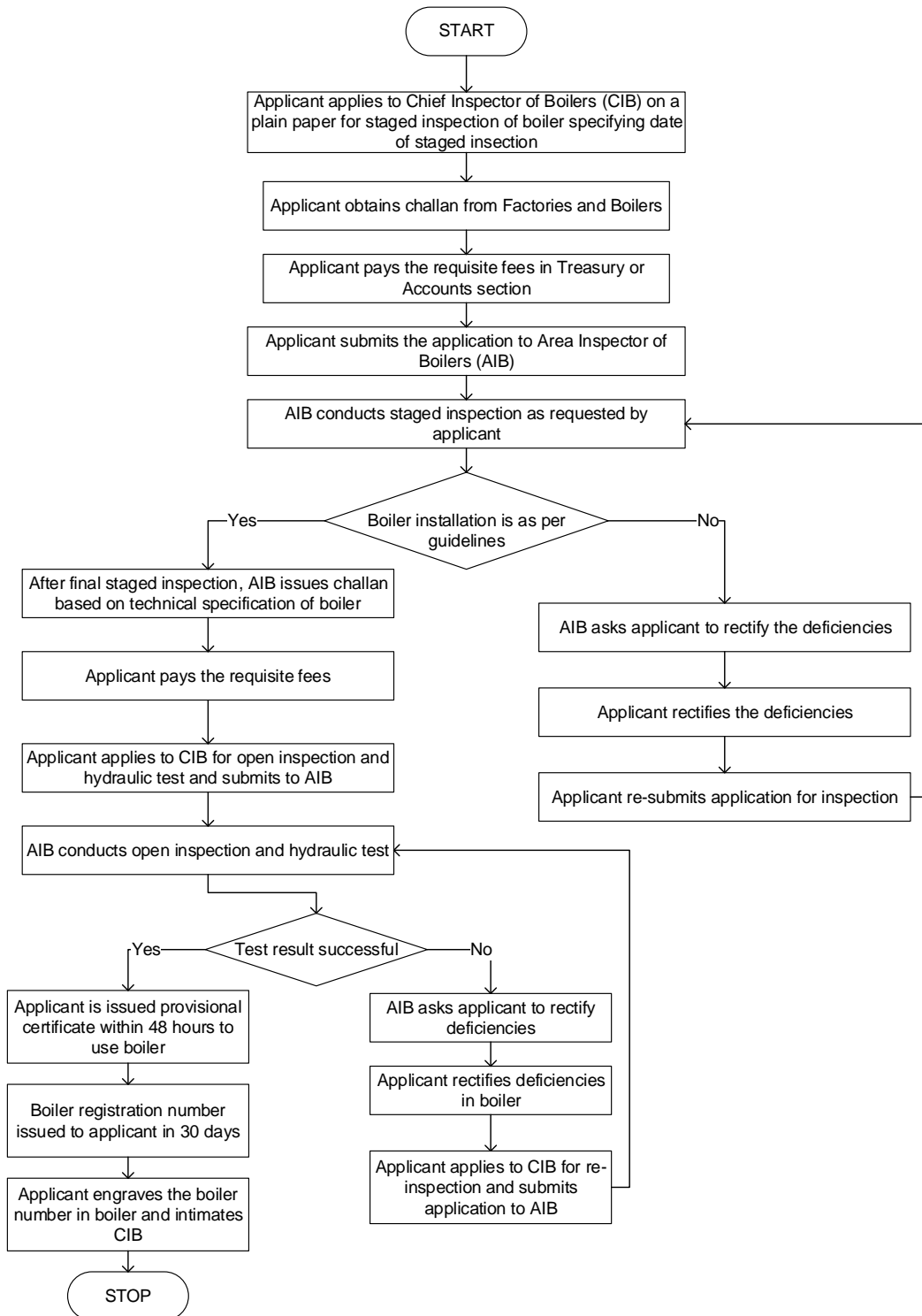
Flowchart: Registration of Boilers – Site Erected Boiler
